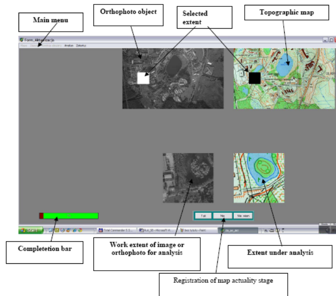
Figure 4. User interface of online map actualization system used to generate bi-sensor/bi-temporal stereopairs.
