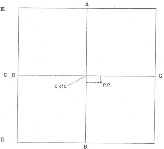
FIG. 12. Schematic drawing showing the principal point with respect to the center of collimation.
