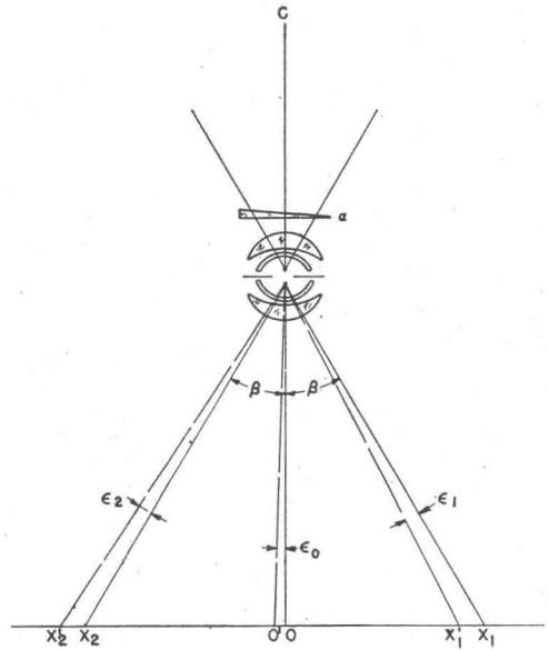
FIG. 10. Schematic drawing showing the image shift produced by interposing a thin prism in front of an ideal lens.
