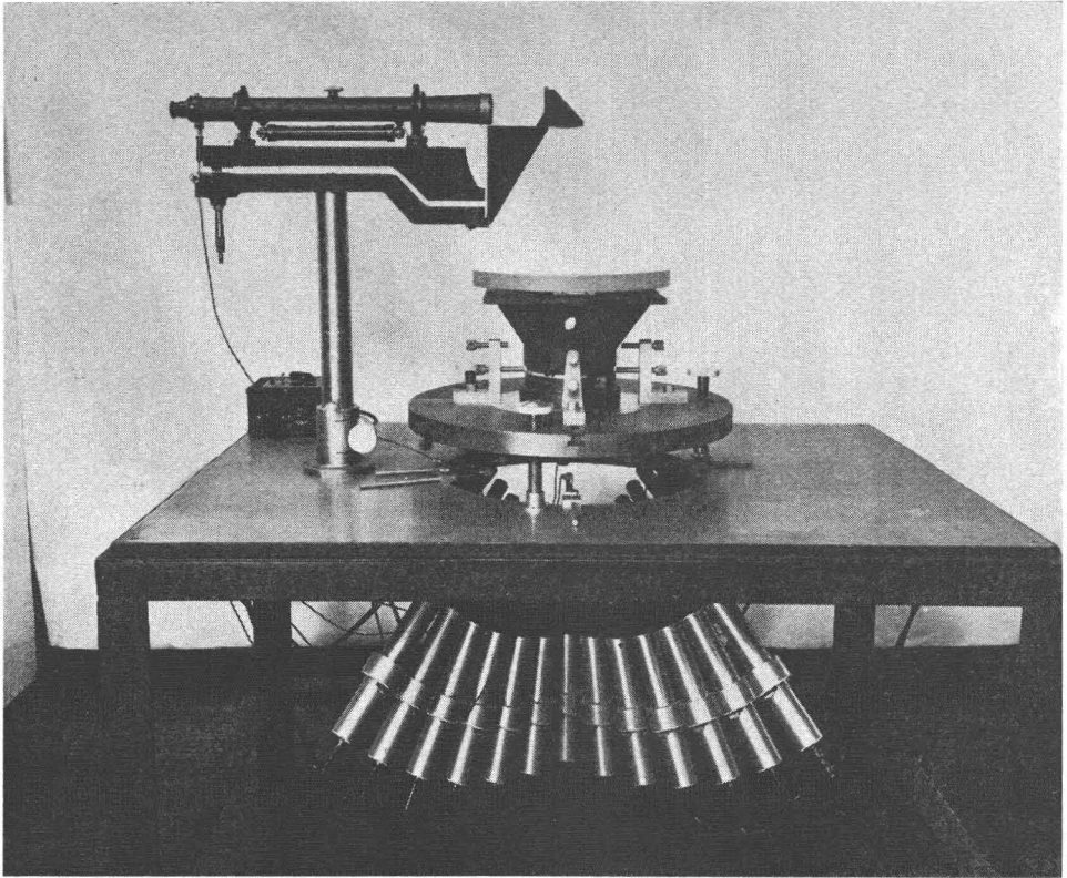
FIG. 2. Photograph of the camera calibrator. This view shows the instrument as arranged for use. The camera under test points vertically downward. Its proper orientation is effected by the auto-collimating telescope and the plane-parallel piece of glass placed on the focal plane of the camera. Images on a finished negative appear every 7.5^\circ along each diagonal, with the collimation index markers registered on each side of the negative.
