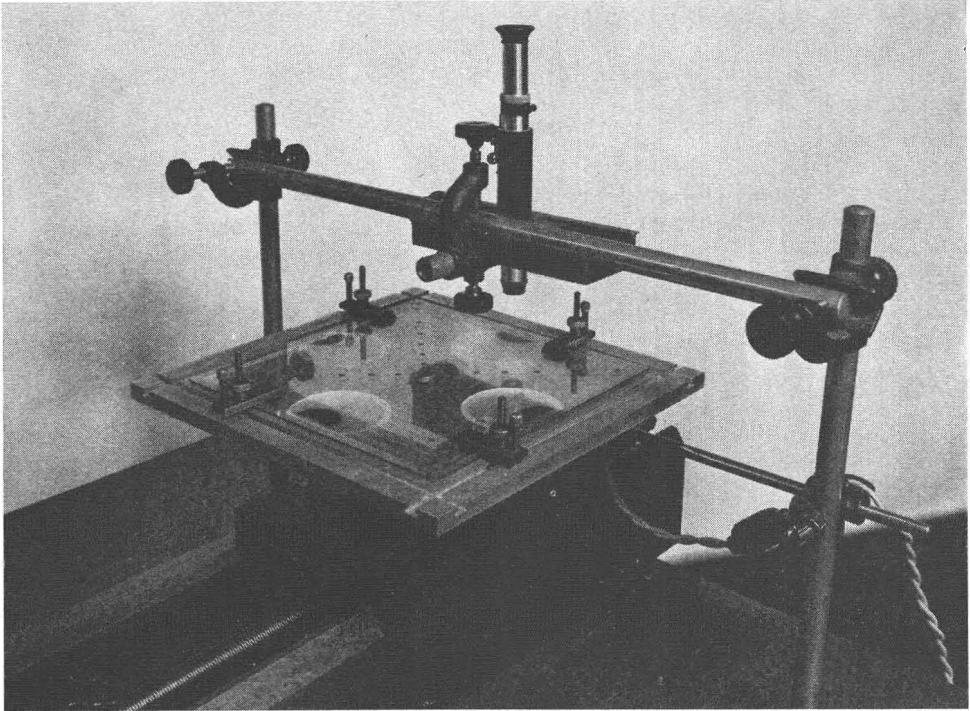
FIG. 7. Photograph of equipment used in the determination of the 90^\circ condition.
