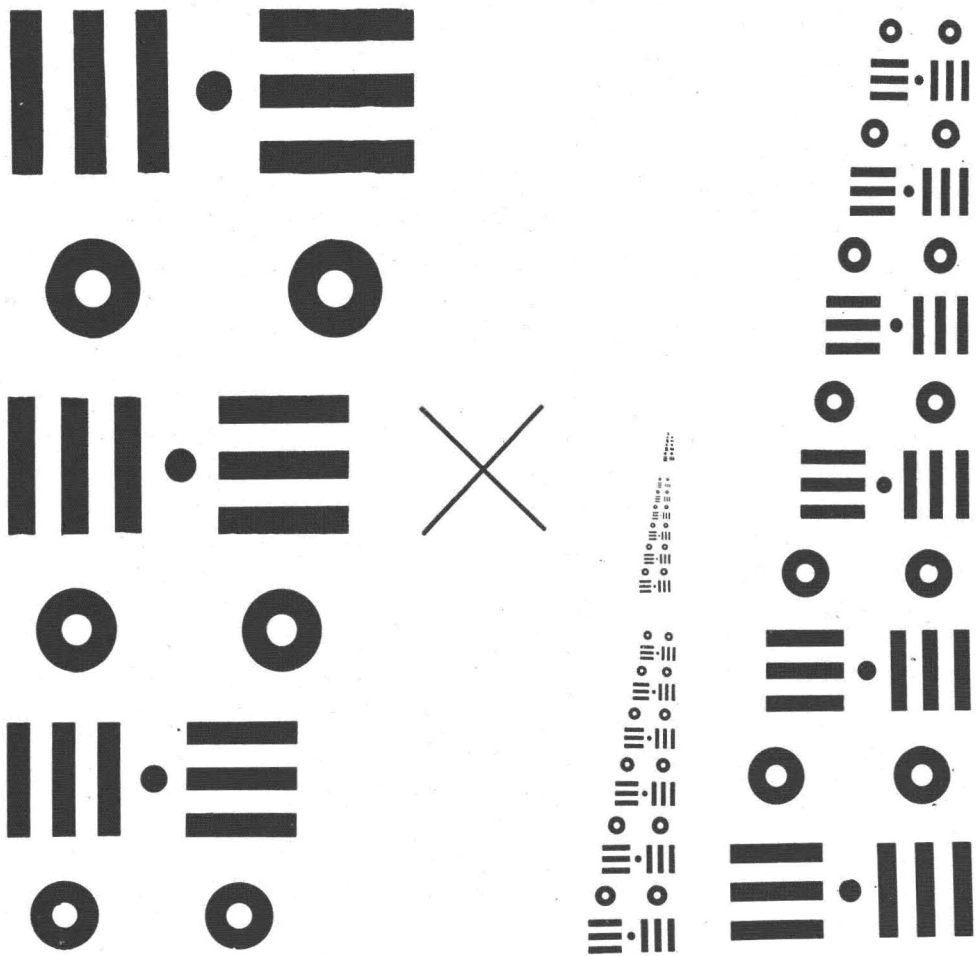
FIG. 3. Test Chart. The test chart which is used in preparing the reticle for use in each collimator consists of patterns of parallel lines in two orientations with spaces varying in geometric progression by steps equal to \sqrt[4]{2} . The circle targets are included for comparative study of line and circle targets.
