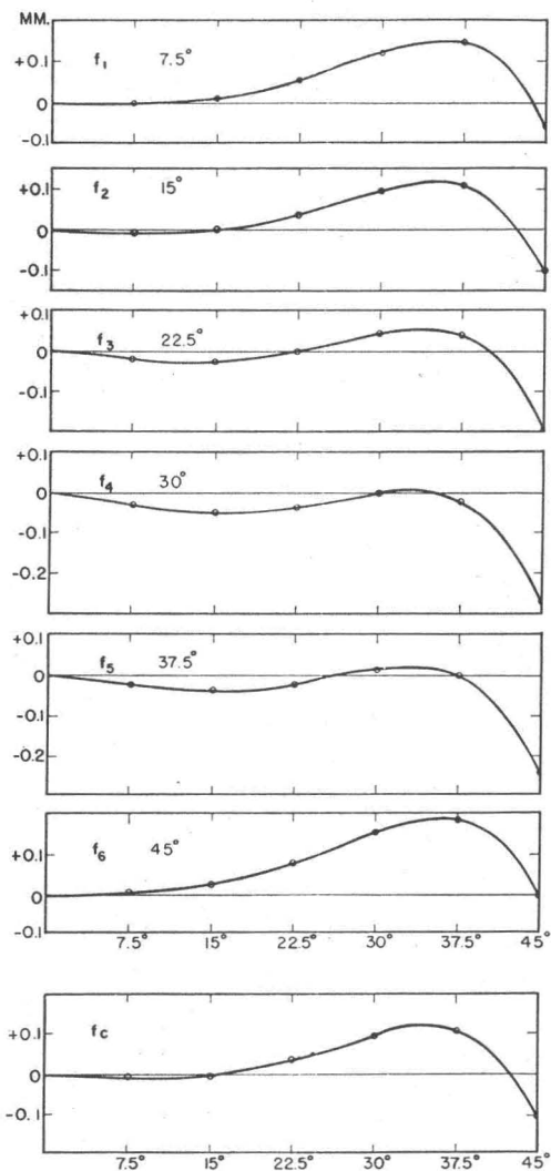
FIG. 13. Variation of distortion in the same image plane with equivalent focal length computed from the relation f = y' / \tan \beta for varying angles of \beta . The lowest curve showing the distortion referred to the calibrated focal length indicates that the calibrated focal length is equal to the equivalent focal length for values of \beta of approximately 16° and 42.5°.
