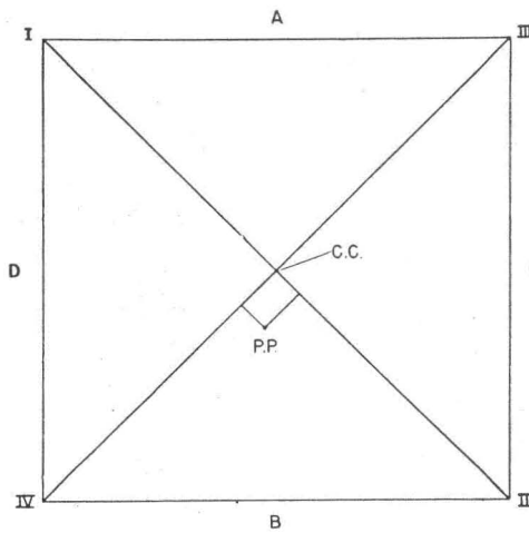
FIG. 11. Schematic drawing showing the principal point with respect to the center cross.
