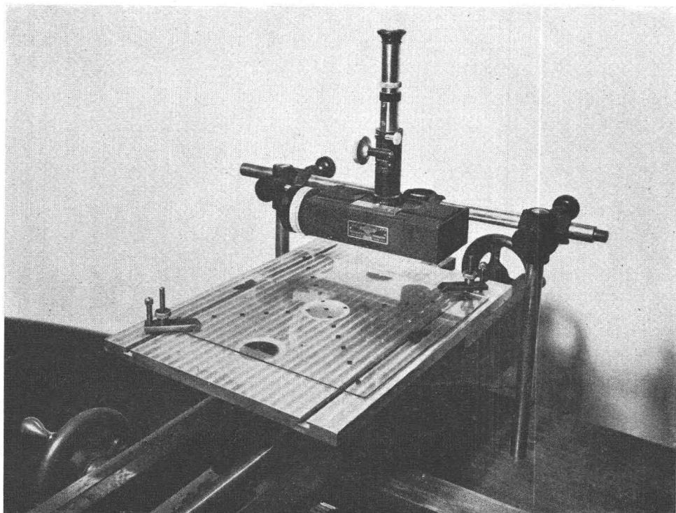
FIG. 8. Photograph of equipment used in locating the center cross with respect to the center of collimation.
