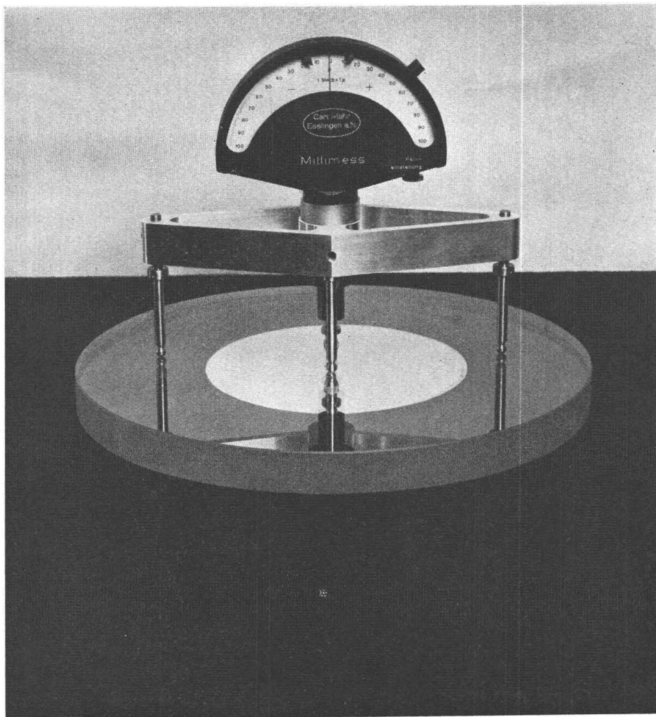
FIG. 14. Photograph of dial indicator device used for checking flatness of platen. The instrument is graduated in microns and permits the rapid measurement of departures from flatness with an accuracy of \pm 0.0001 inch.
