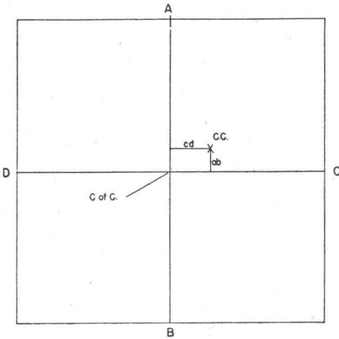
FIG. 9. Schematic drawing showing the center cross with respect to the center of the collimation.
