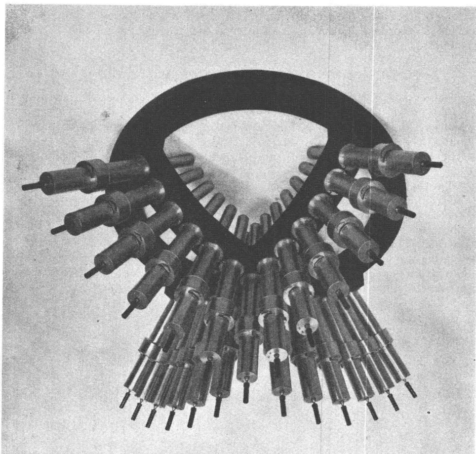
FIG. 1. Collimator bank of camera calibrator. The photograph shows a view of the collimator bank before installation in the instrument. It consists of 25 collimators arranged in the form of a cross. When mounted in the camera calibrator, the central collimator points vertically upward with the remaining 24 collimators spaced at 7.5^\circ intervals along the two meridians. Accuracy of pointing of the collimators depends upon the special casting in which they are mounted.
