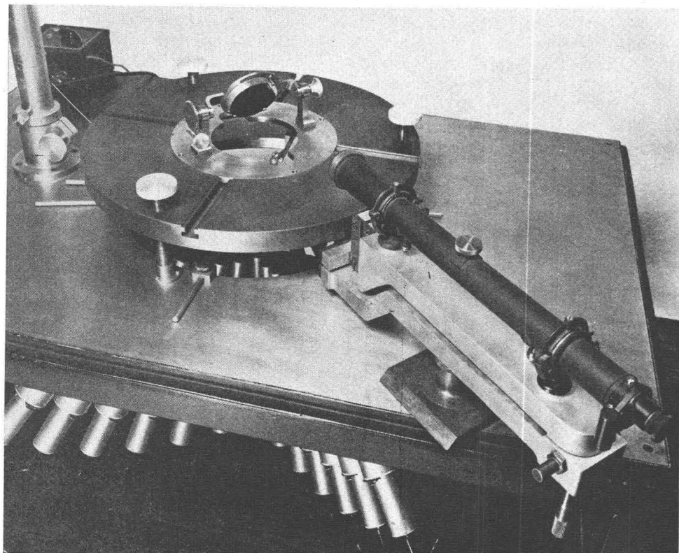
FIG. 5. Photograph showing reflecting biprism for measurement of angles.
