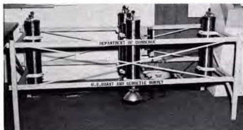
FIG. 5. Narrow frame Model B deep-sea camera configuration.
