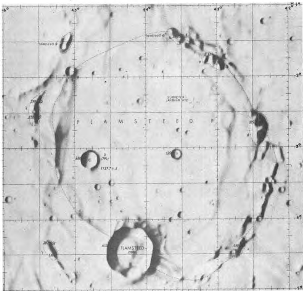
FIG. 1. Surveyor I spacecraft landed near lat 2.52^{\circ} S. and long 43.34^{\circ} W. on the nearly buried floor of the large Flamsteed P crater.
