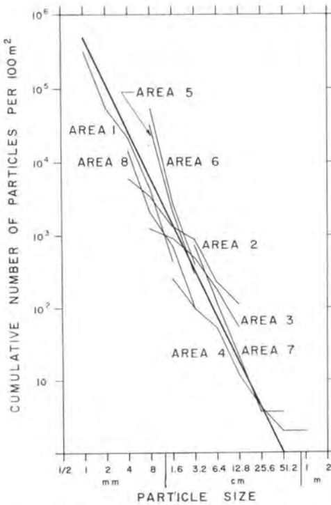
FIG. 14. Cumulative size-frequency distribution of particles on lunar surface as determined from Surveyor I pictures.
