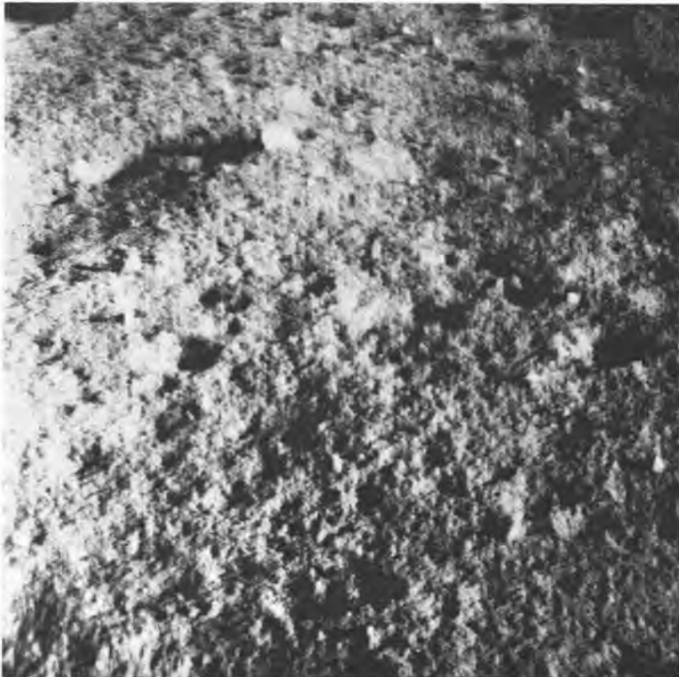
FIG. 7. Area A illuminated at sun elevation angle of approximately 20°.
