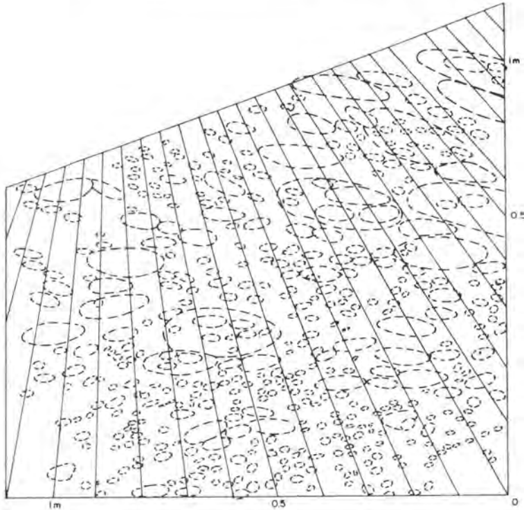
FIG. 8. Sketch map of craters counted and measured in Area A.
