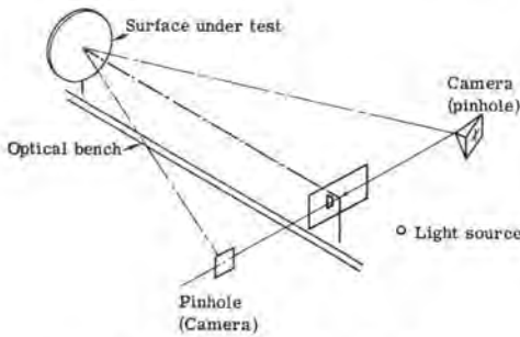
FIG. 6. Stereo-Foucault setup.
