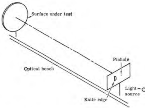
FIG. 4. Laboratory setup for the Foucault test.
