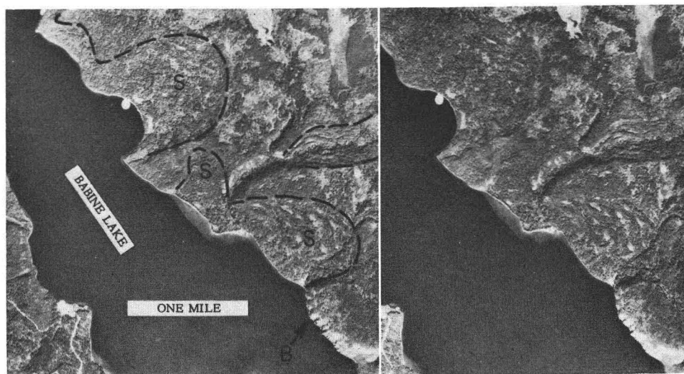
FIG. 1. Massive slumps and earth flows S have occurred in deep glacial materials on the north side of Babine Lake in British Columbia. A nearby bluff of columnar basalt B shows no sign of instability. Deep glacial materials consist of glacial till and lakebed sediments. These materials were deposited against glacier ice which occupied Babine valley during melting of the glaciers. Canadian Government Airphoto.
