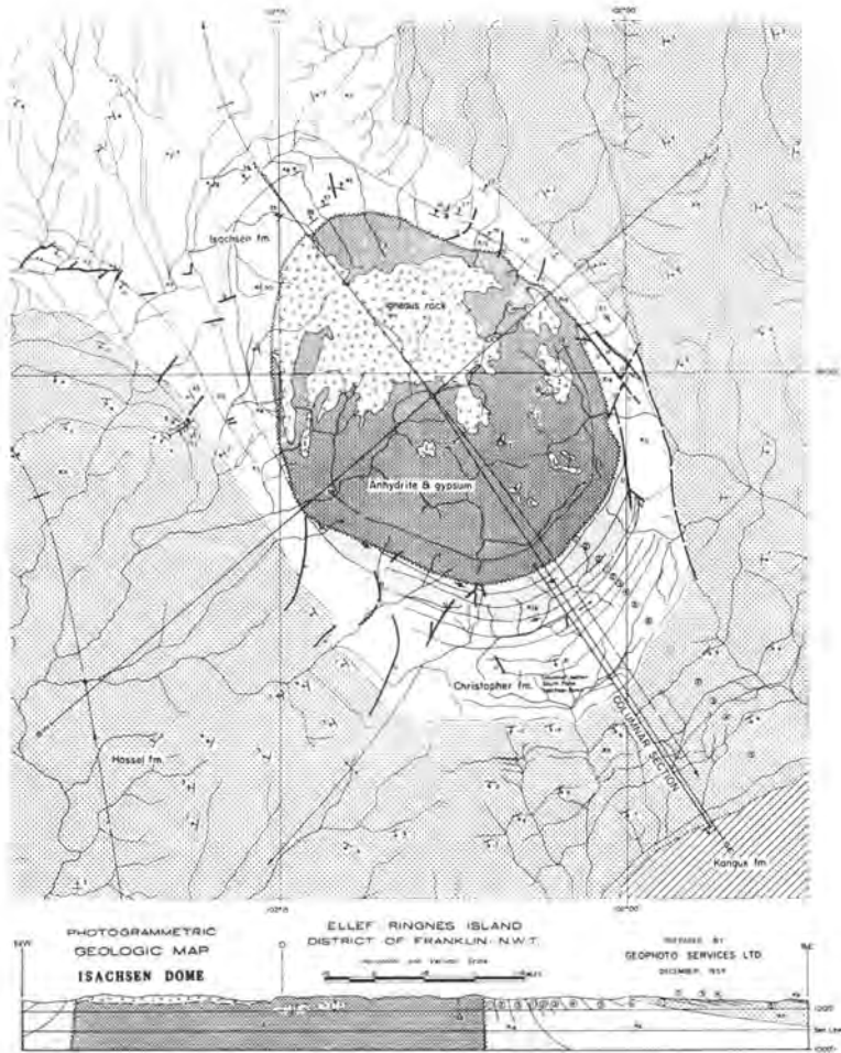
FIG. 2. Photogrammetric geologic map and cross-section of Isachsen Dome prepared from aerial photographs.
