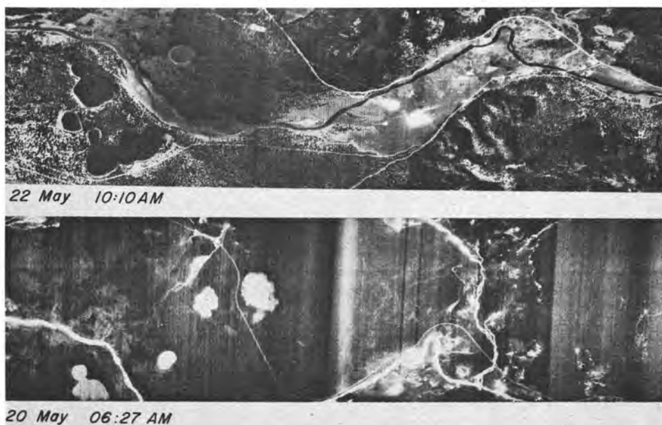
FIG. 3. Infrared imagery of Midway Geyser Basin. The differences in the imagery demonstrate the diurnal change in radiation pattern of the terrain from early to late morning.
