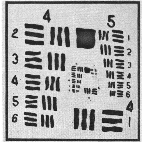
FIG. 6. Resolution from 7.85-inch lens: 128 lines/mm., 20^\circ tilt.
