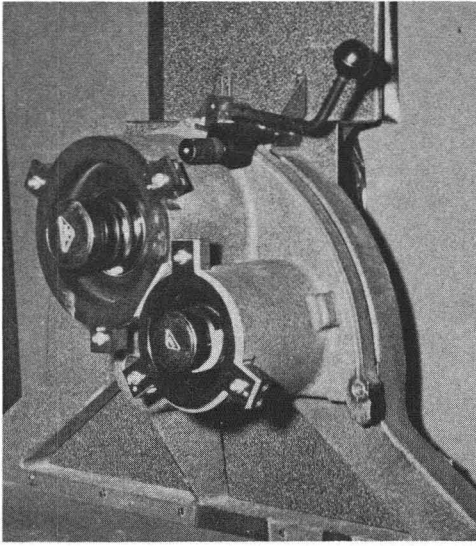
FIG. 5. Lens carriage.
