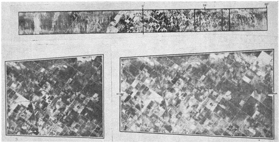
FIG. 10. Segmented Panoramic Rectification. Top : Contact print, f=12 inches, Arizona Test Area. Left : Frame program. Right : Panoramic program.
