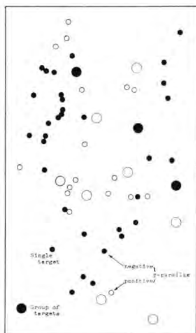
FIG. 1. Residual Y -parallaxes in Model M_1P_{12} .
