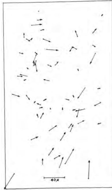
FIG. 2. Projections of residual position vectors on the XY -plane.
