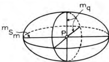
FIG. 12. The ellipsoid of errors. Point P corresponds to point P in Figure 11, and m_{sm} is in the direction of MP in Figure 11.
