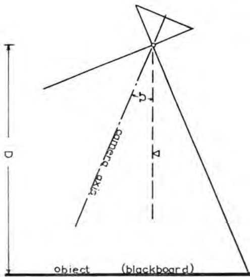
FIG. 9. Tilted photograph.
