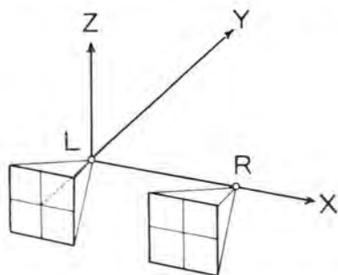
FIG. 6. Camera coordinate system. In the test apparatus described in Section 3.1 the Y -axis took a vertical direction pointing downward.
