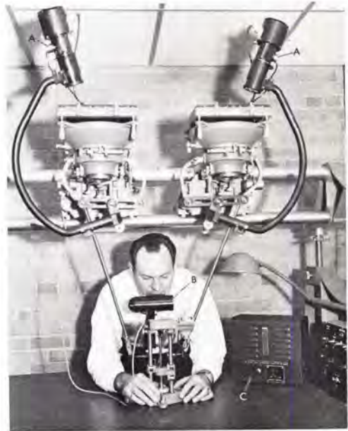
FRONTISPIECE. The Stereolmage Alternator system installed on Kelsh K-100 plotter. A —projection shutter motors. B —viewing shutter assembly. C —control logic unit.
