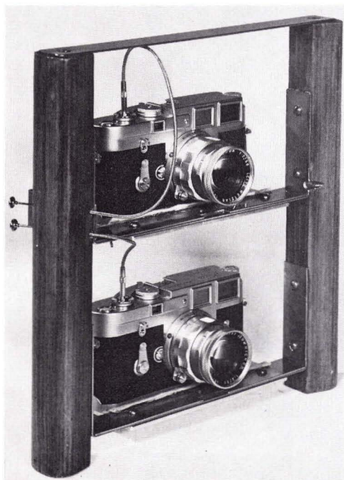
FIG. 10. Paired camera arrangement for making simultaneous photographs.
