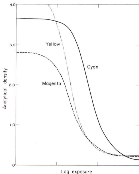
FIG. 3. Sensitometric curves.
