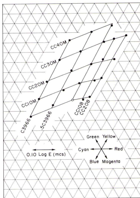
FIG. 8. Color shifts produced by various combinations of Kodak Color Compensating and Corning No. 3966 filters.
