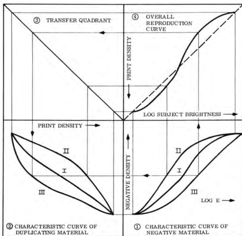
FIG. 3. A tone-reproduction curve for three spectral photographs showing the relationship between regional scene and the final positive reproduction.
