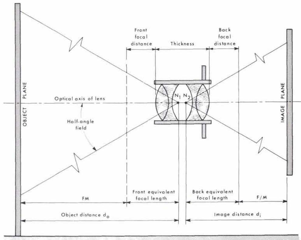
FIG. 1. A photographic objective showing the optical constants and the relation between the object and image distances.
