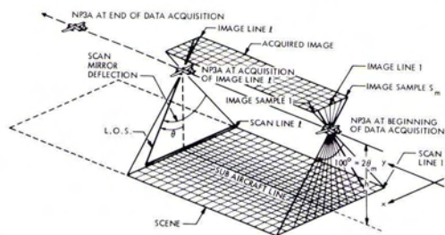
FIG. 3. Geometry of electronic scanner images.
