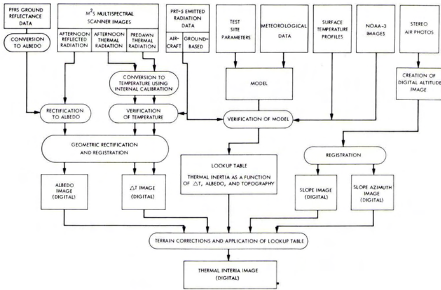
FIG. 1. Data processing diagram.
