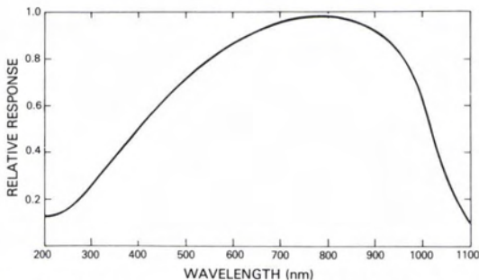
FIG. 3. Response curve of a typical detector element between 200 and 1100 nm.
