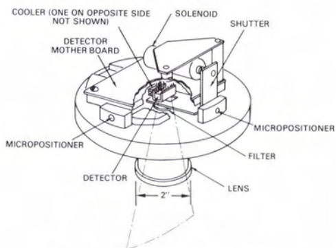
FIG. 2. Diagram of a LAPR sensor.
