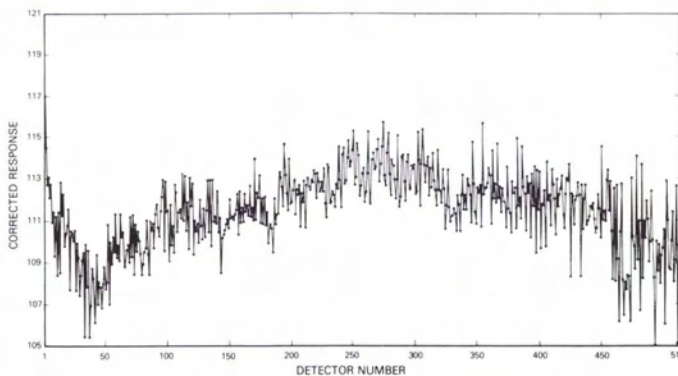
FIG. 4. Plot of the corrected response vs. detector number for a spectral radiance level of 7.09 \mu\text{W}/\text{Ster}/\text{cm}^2/\text{nm} .
