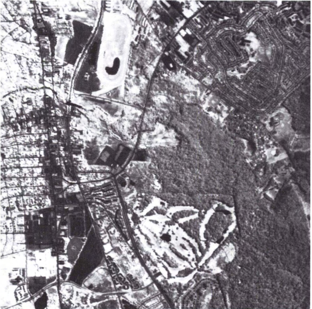
FIG. 5. Channel 1, near-infrared (802.5-847.5 nm) LAPR image collected over Laurel, Maryland.
