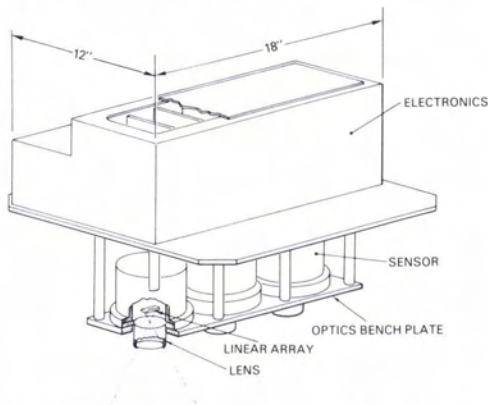
FIG. 1. Structural components of the LAPR instrument.
