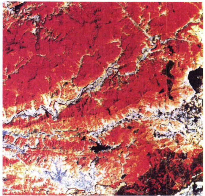
PLATE 1. Infrared composite of L3122-I 1:50,000-scale map area (50-metre resolution).
