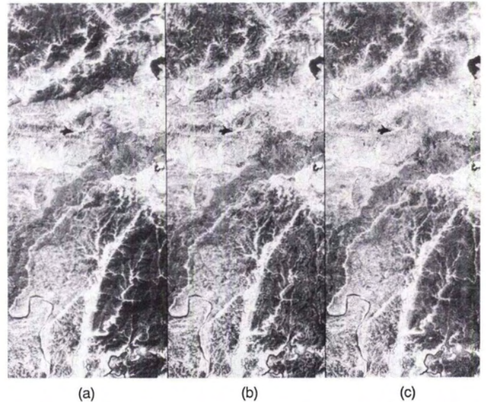
FIG. 1. TM band 3 uncorrected data (a), corrected using DEM level I (b), and corrected using DEM level II.
