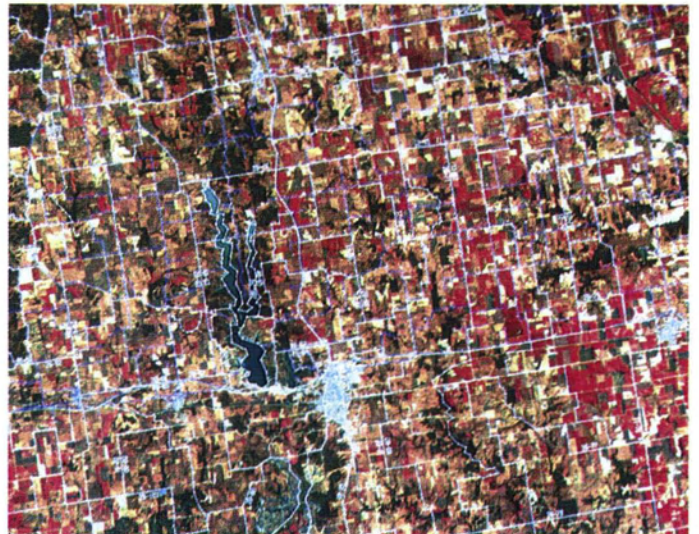
PLATE 1. DLG and PSU boundaries. A 1024- by 1280-pixel window of a TM image of Macon County was displayed using channels 2, 3, and 4 in blue, green, and red, respectively. Therefore, the highly vegetated areas appear to be dark red. Using the two graphic overlay planes, DLG transportation systems were overlaid in blue, and the boundaries of the PSUs were overlaid with strata labels in white.
