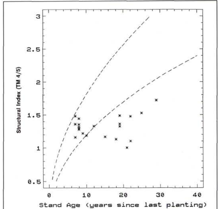
Figure 2. The relationship between the Structural Index, SI (TM 4/5 ratio) and the age of poorly regenerated conifer stands where the understory is predominately herbs (herb stands) (n = 21 from 20 stands). The prediction interval from the regression of well regenerated stands (Figure 1) is included to illustrate the differences between herb stands and well regenerated stands. Age is determined from the most recent planting date.
