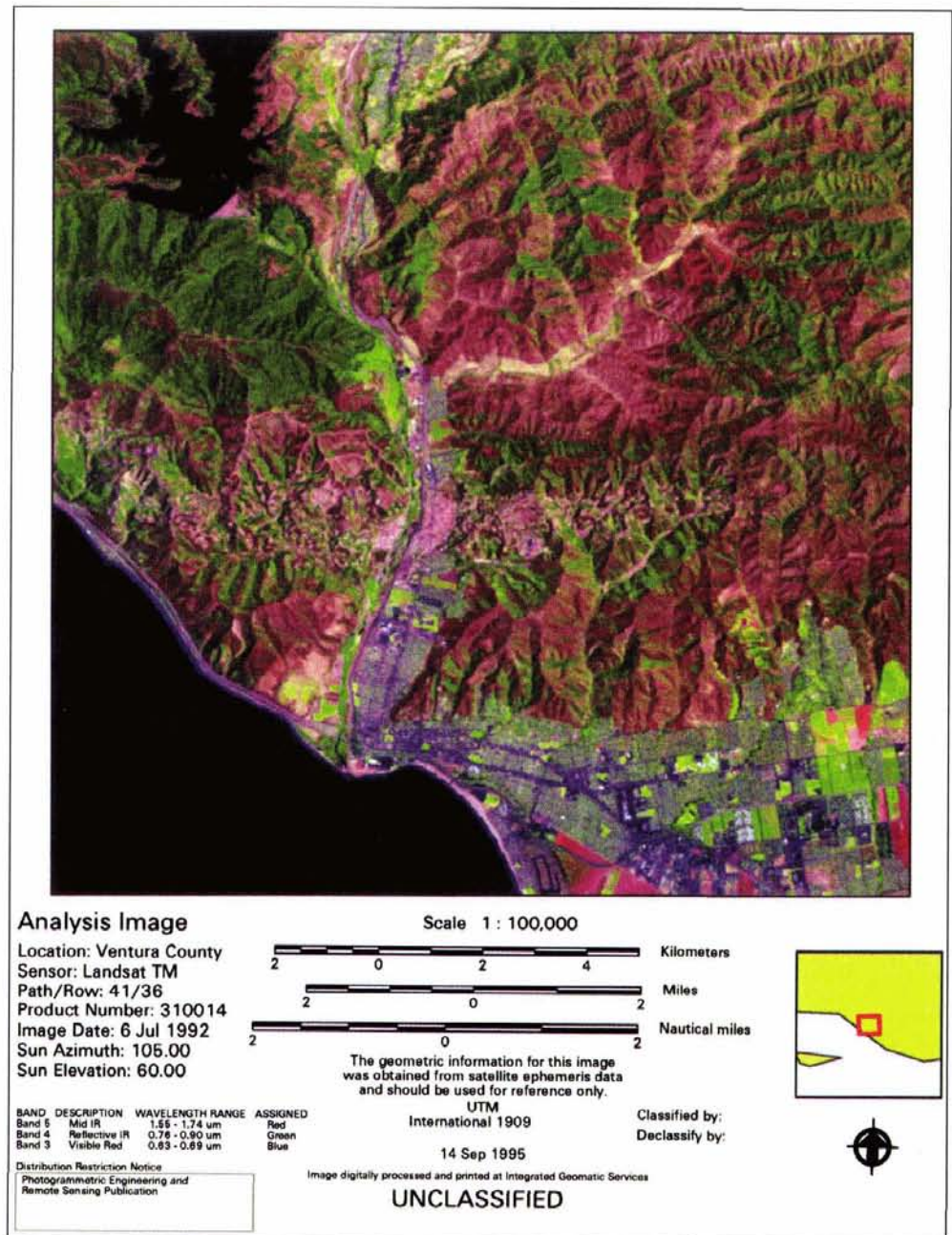
Figure 1. Example Analysis Image Product created using CPG. The product is a 1:100,000 scale subsense of a Landsat Thematic Mapper Image of Ventura County, California using a Short Wave Infrared band combination (5,4,3). The image was enhanced using a standard equal area stretch to each of the three bands. The marginalia displayed in the product is part of the product format and automatically generated from image header data.
